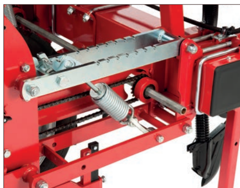
Molla supplementare elemento Additional spring pressure element
